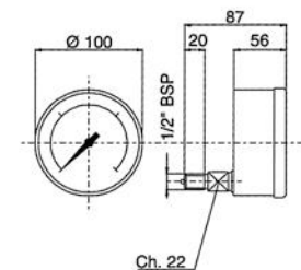
Assiale / Axial MAA-100
